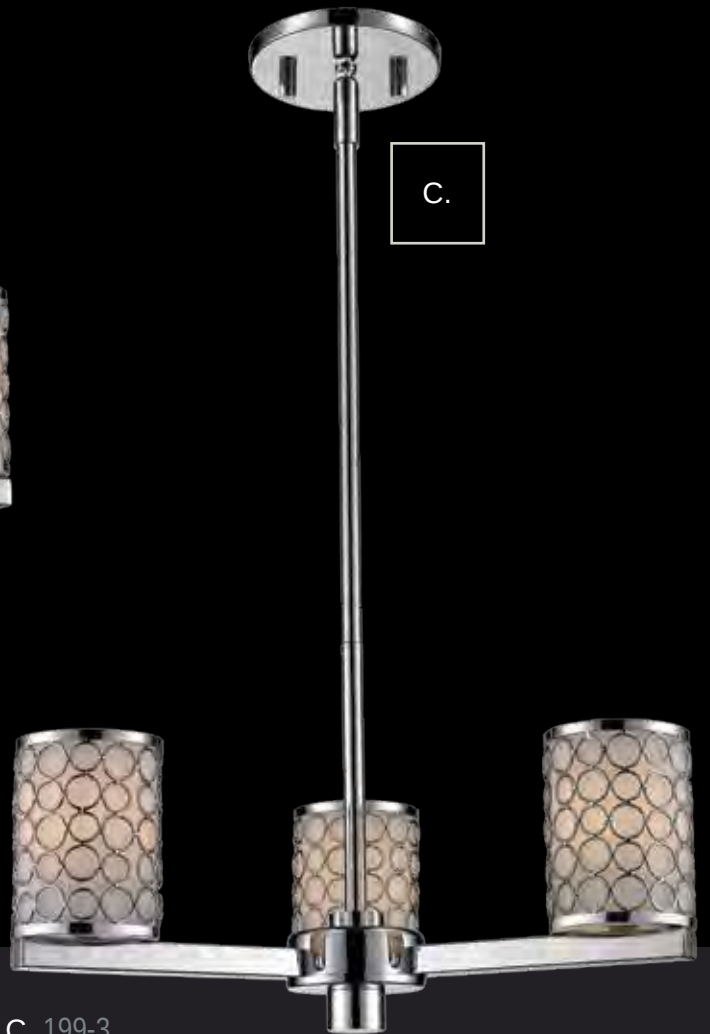
C. 199-3 11 7/8"W x 50"H includes: 3x12"+ 1x6"+1x3" rods adjustable to suit height 3-40w/G9 (included)
